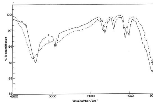
Fig. 4 FT-IR spectra of a) BTBA and b) BTBA-Cu complex
