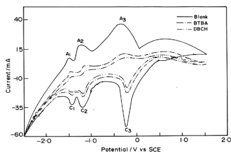
Fig. 3 Cyclic voltammograms of brass in 0.5 M NaCl solution containing optimum concentrations of BTBA and DBCH
