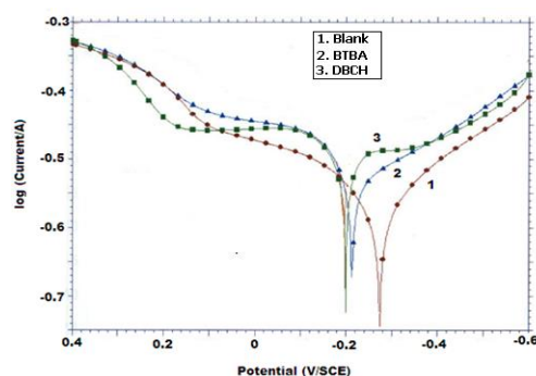
Fig. 1 Polarization curves for brass in 0.5 M NaCl solution containing optimum concentrations of BTBA and DBCH
