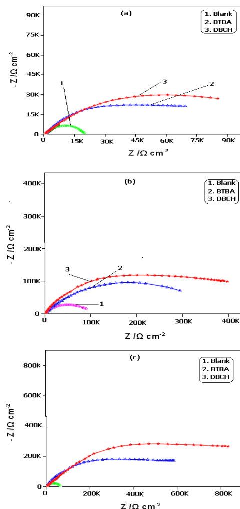
Fig. 2 Nyquist diagrams for brass in 0.5 M NaCl solution containing optimum concentrations of BTBA and DBCH after immersion of (a) 1h (b) 24hrs and (c) 48hrs
