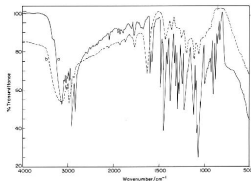
Fig. 5 FT-IR spectra of a) BTBA and b) DBCH-Cu complex
