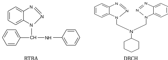
Scheme 1 Structure of organic inhibitors
