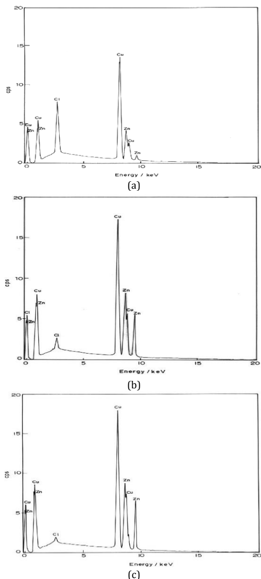
Fig. 6 (a) EDX spectrum of brass in 0.5 M NaCl solution (b) EDX spectrum of brass in 0.5 M NaCl solution containing optimum concentration of BTBA (c) EDX spectrum of brass in 0.5 M NaCl solution containing optimum concentration of DBCH
